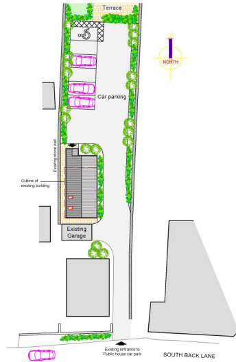
PROPOSED SITE PLAN Scale 1:200
